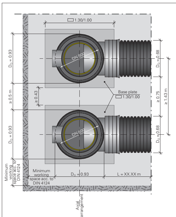
Axial arrangement
