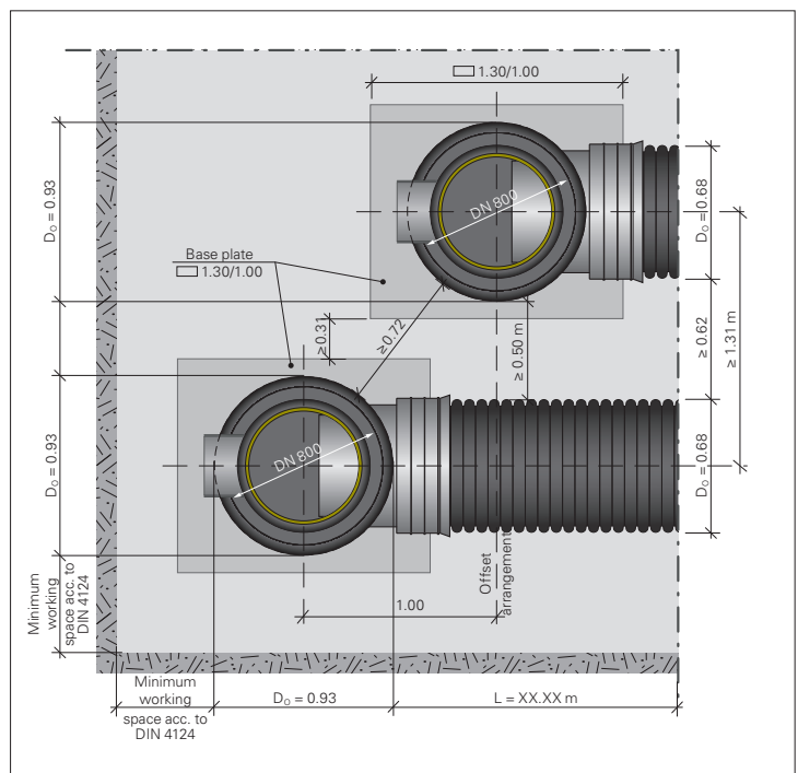
Offset arrangement
