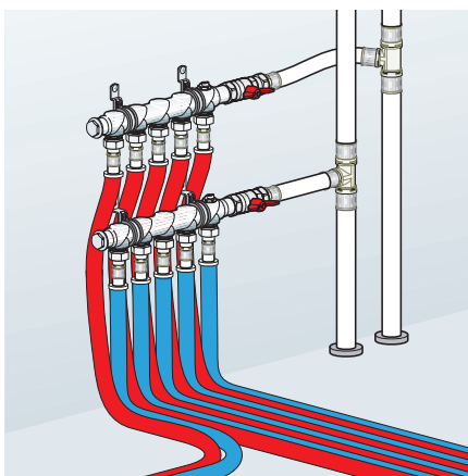
Mounting of the manifold to the building structure
