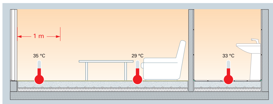
Max. surface temperature in rooms with heated floors
