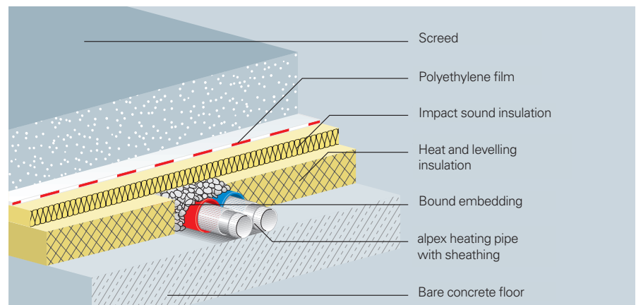
Floor structure under screed with alpex pipe and appropriate sheathing
