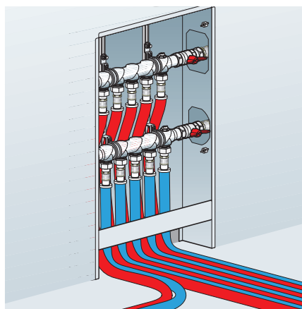
Mounting of the manifold in the manifold cabinet
