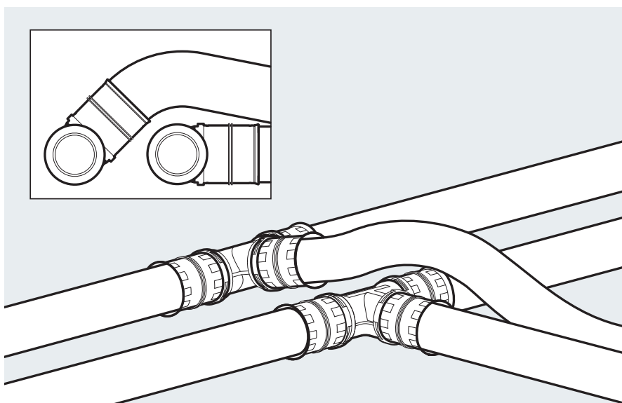
Tee installation with pipe bridge using alpex systems
