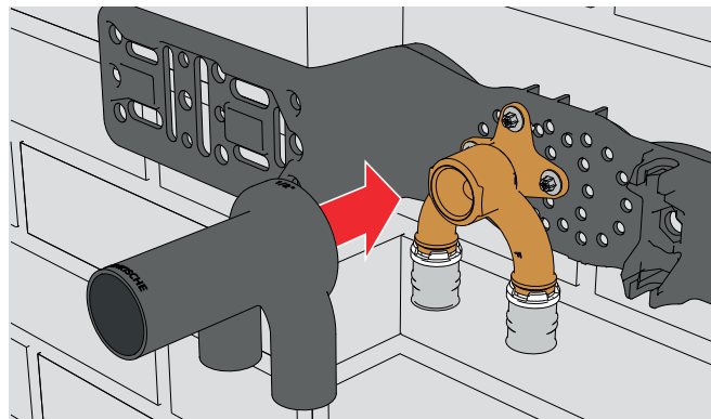
alplex sealing for double wall mount elbows
