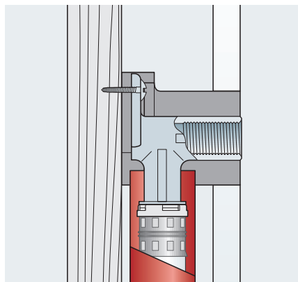
alpeX wall mount elbow
