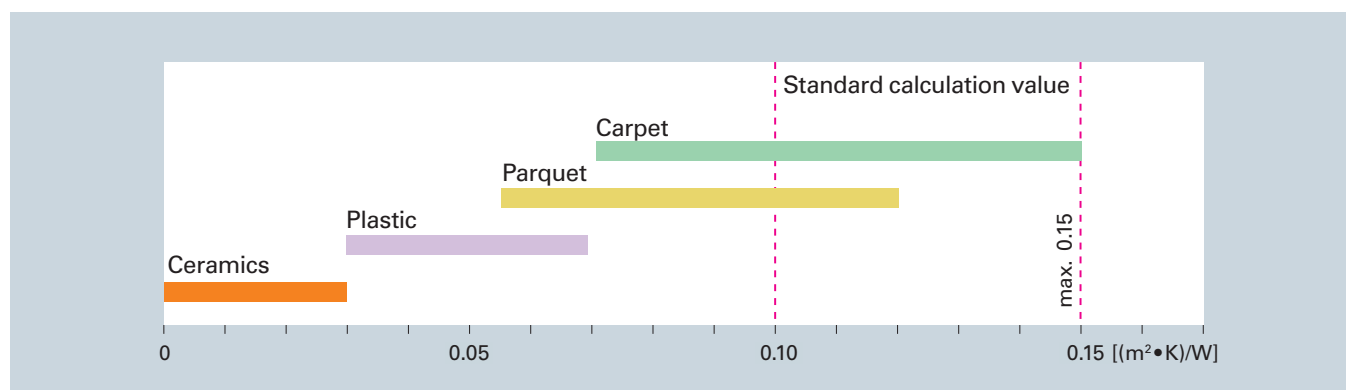
Overview of thermal resistances
