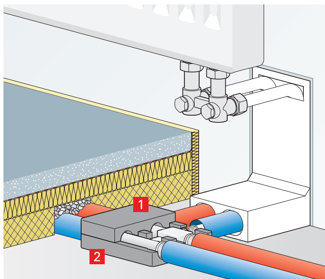
1 acoustic isolation from the screed slab
