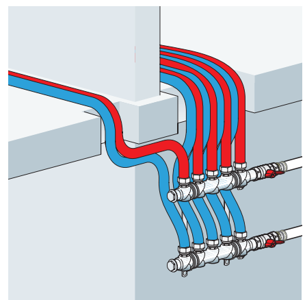
Mounting of the manifold beneath the basement floor
