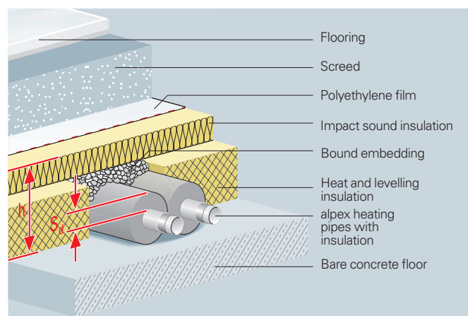
Floor structure with pipe insulation
