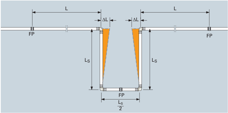
Compensation for length change using a U-shaped expansion bend
