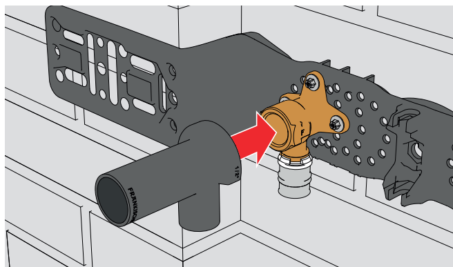
alplex sealing for wall mount elbows
