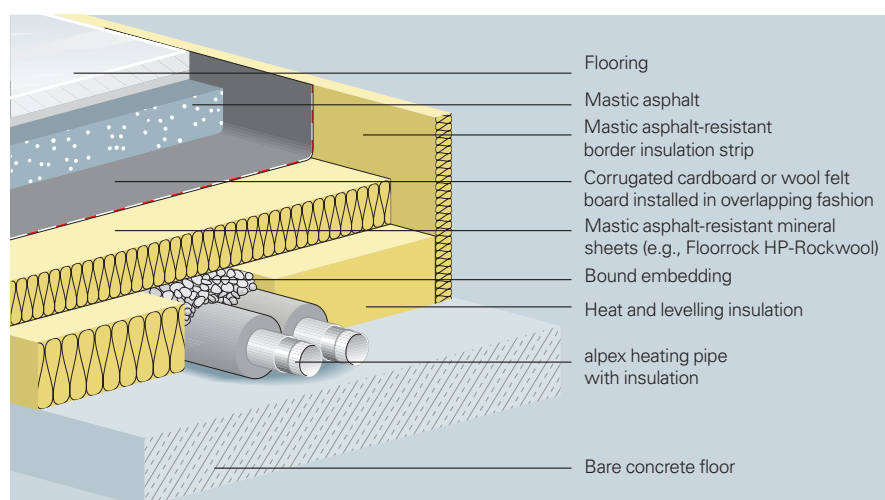
Floor structure under mastic asphalt
