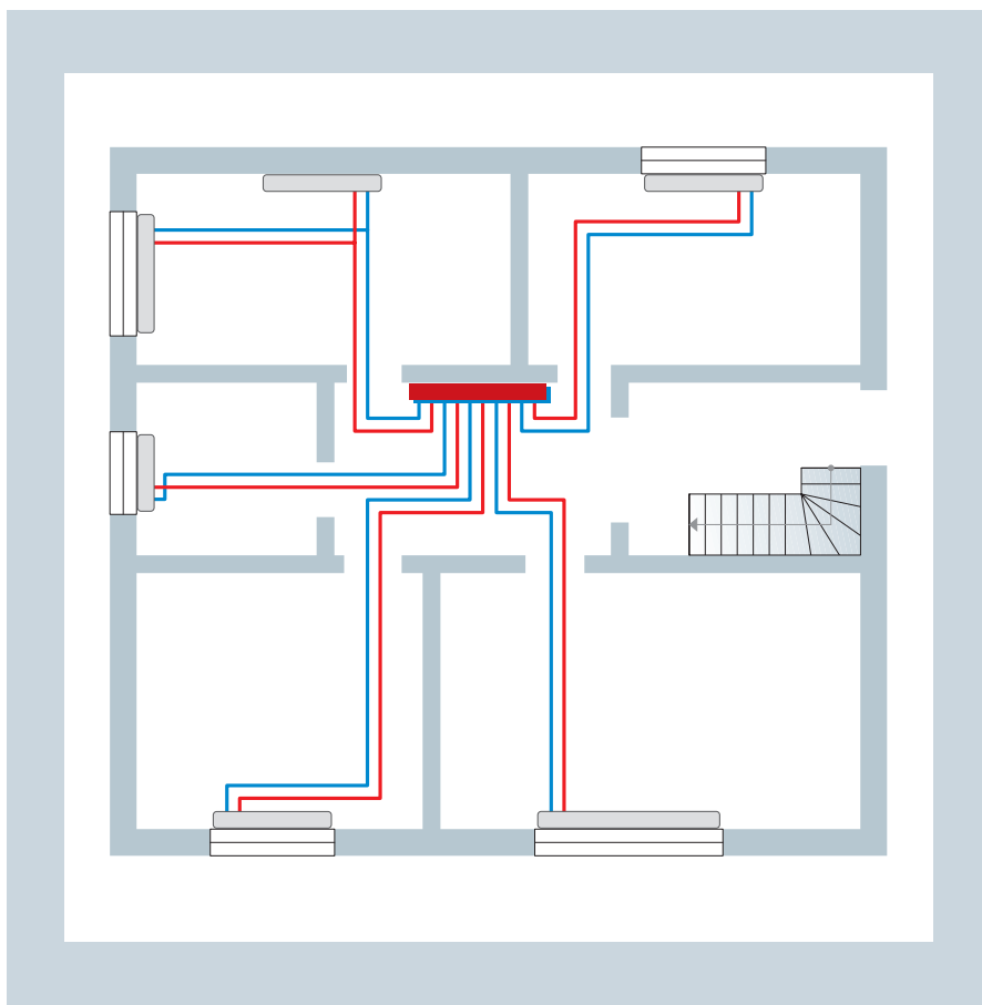
Floor plan with heating circuit routing
