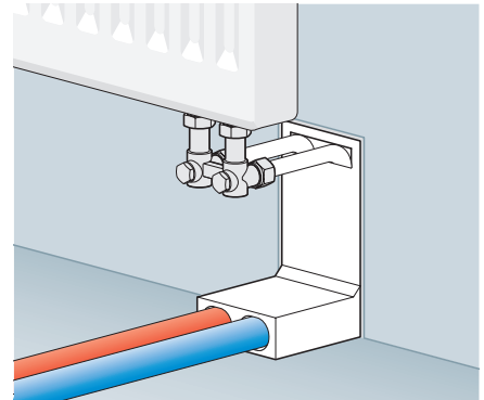
alpex single connection from manifold with radiator connection block
