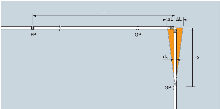
Compensation for length change using an expansion bend "L s "
