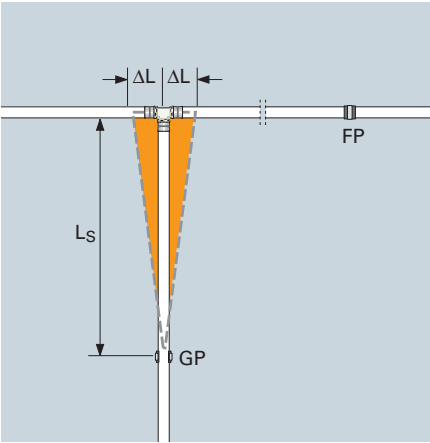
Compensation for length change with an expansion bend "L s "
