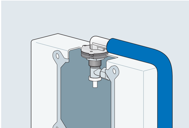
alpeX concealed toilet cistern elbow
