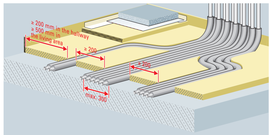
Pipe run widths and supporting area widths
