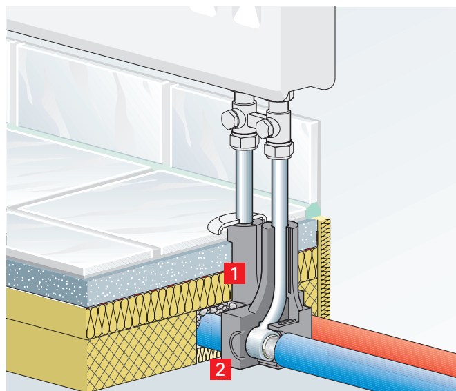
2 acoustic isolation from the bare concrete
