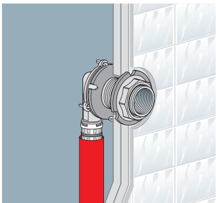
alpeX wall feed-through in light-weight construction
