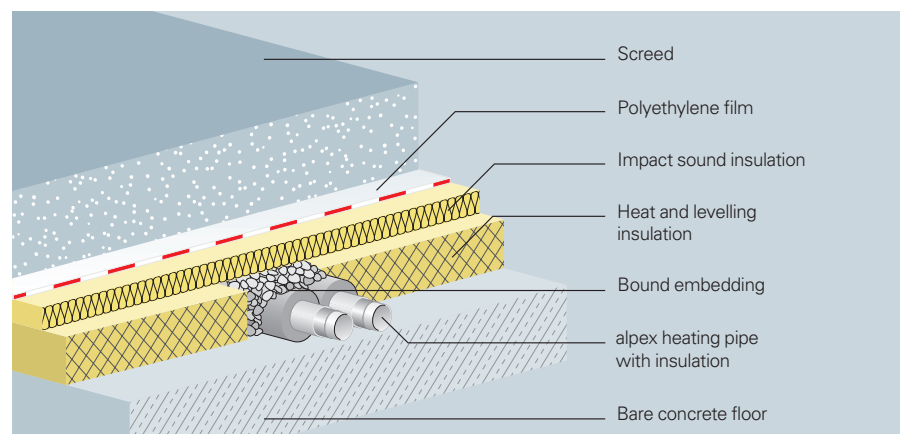
Floor structure under screed with pre-insulated alpex pipe
